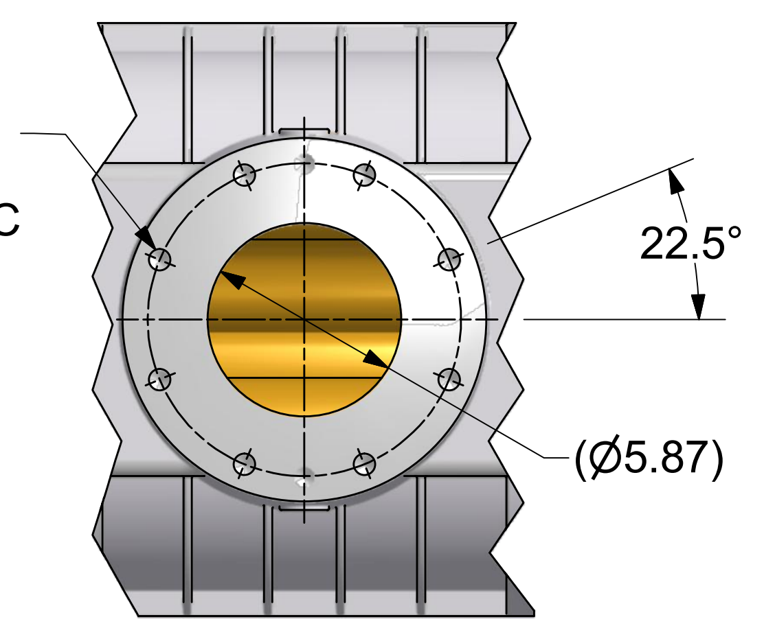
VIEW B-B SCALE 1 / 4
